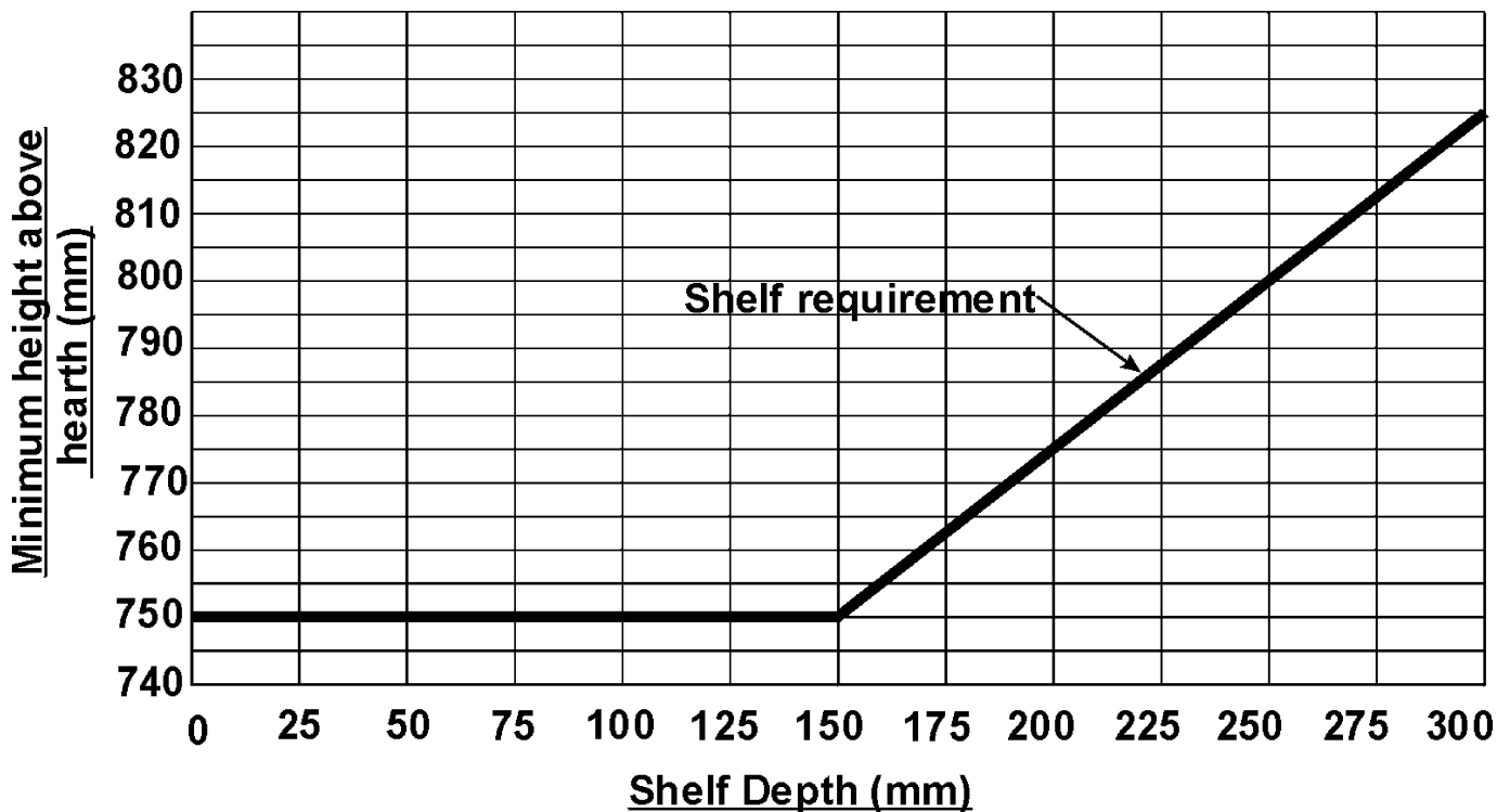
Graph 1. Combustible shelf clearances
