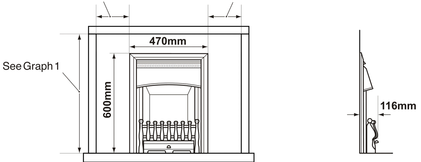
Figure 1. Appliance dimensions
